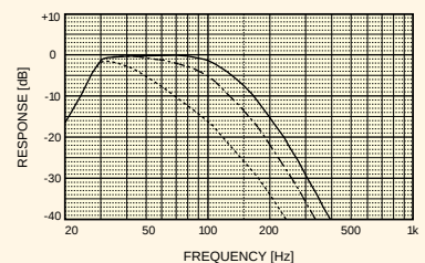
SW10 Frequency Response
